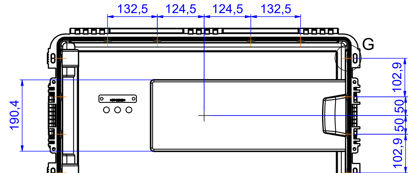
INTERNAL VIEW BOTTOM
