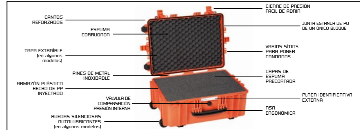
9413 ■■■ Dim. Int. 939x352x137 mm. 36 15/16 x 13 7/8 x 5 3/8 in 11413 ■■■ Dim. Int. 1136x350x135 mm. 44 3/4 x 13 3/4 x 5 5/16 in 13513 ■■■ Dim. Int. 1350x350x135 mm. 53 1/8 x 13 3/4 x 5 5/16 in 13527 ■■■ Dim. Int. 1350x350x272 mm. 53 1/8 x 13 3/4 x 10 11/16 in 15416 ■■■ Dim. Int. 1540x377x160 mm. 60 5/8 x 14 13/16 x 6 5/16 in
